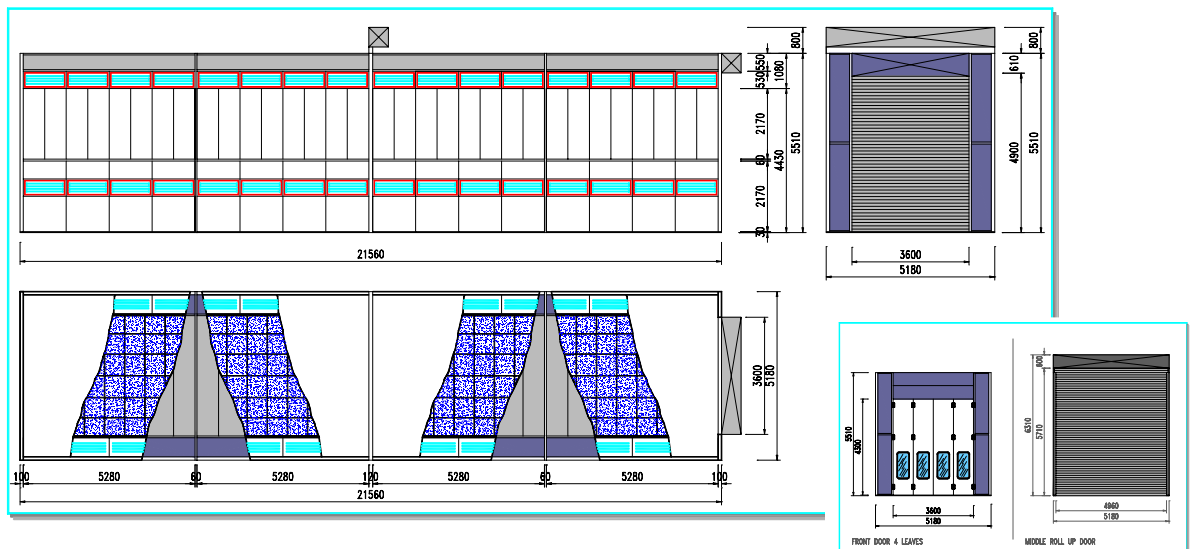
INDICATIVE DRAWING
