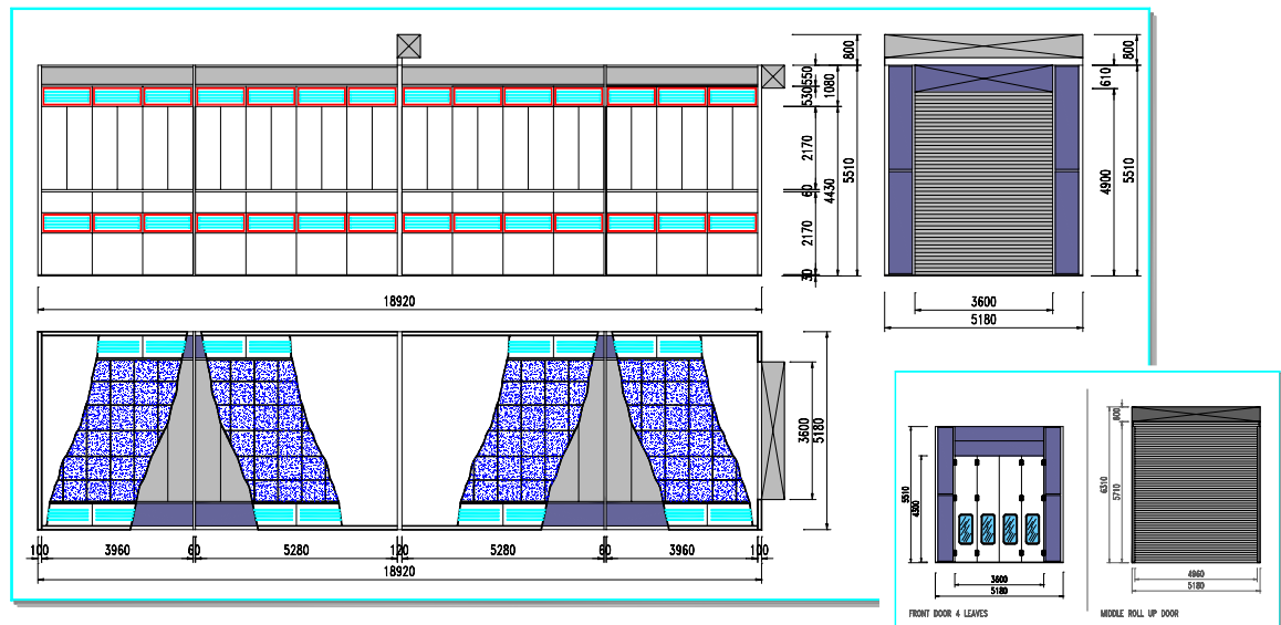
INDICATIVE DRAWING
