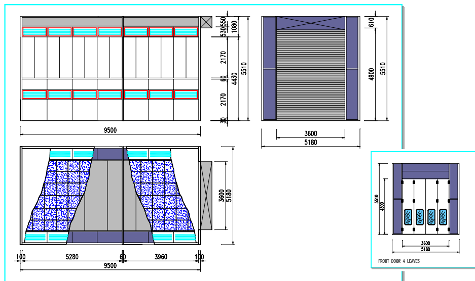
INDICATIVE DRAWING
